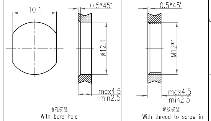
面板安装尺寸 Panel Cut-out
