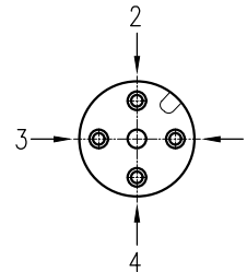
针位图 Contact arrangements
