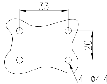
面板开孔尺寸 Panel opening size
