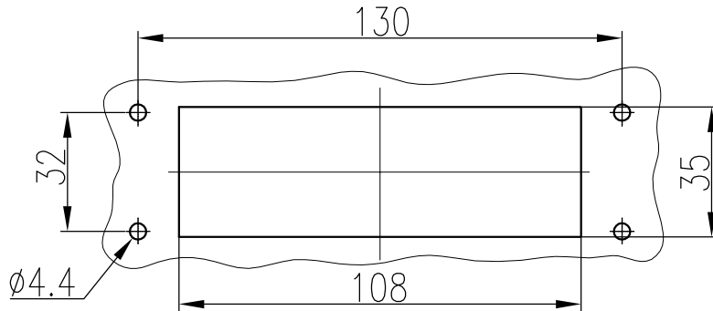
面板开孔图 Panel cut out
