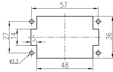
面板安装开孔图 Panel cut out
